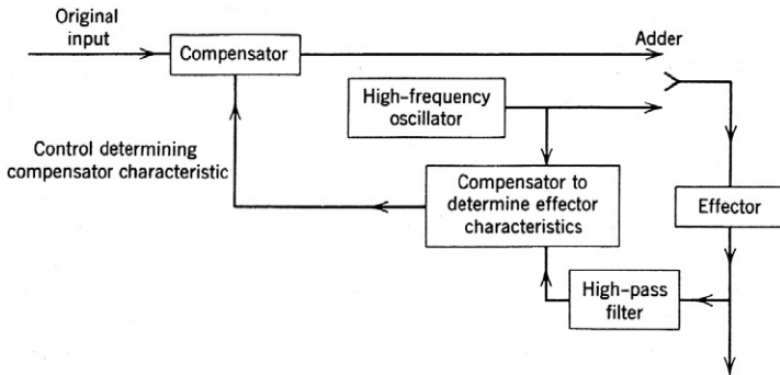
Figure 0.3 Feedback system 17
